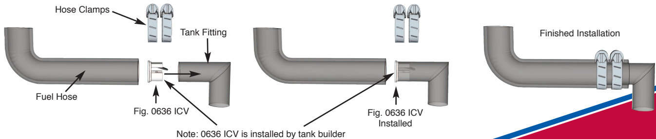
Fig. 0636 for 1-1/2" Fuel Tank Inlet Fittings
